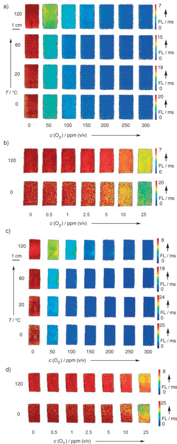
Figure 2. Pseudocolored fluorescence lifetime (FL) images of C_{70} in organosilica (a,b) and C_{70} in ethyl cellulose (c,d) between 0 and 120°C and O_2 concentrations from 0 to 300 ppm in nitrogen at atmospheric pressure (dark red: maximum FL; dark blue: zero). Parts (b) and (d) are exemplary measurements at oxygen concentrations in the low-ppm range.
